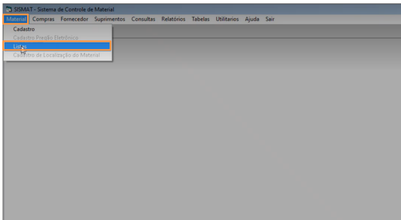
Figura 1 – Menu Material
